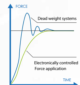
Load cell, closed loop, force feedback system
