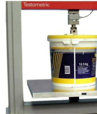
Compression Testing
