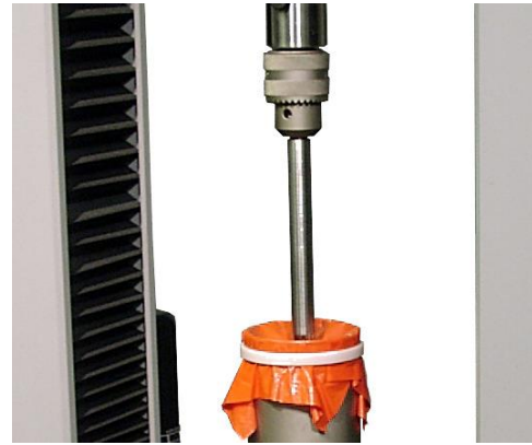
Puncture Testing
