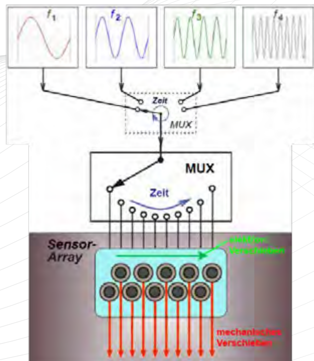
Combination of parameter multiplex with sensor multiplex
