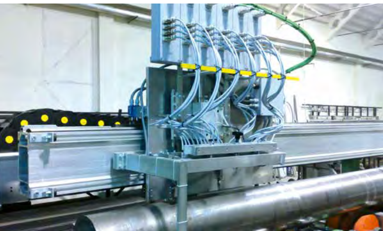
Tube inspection with probe array
